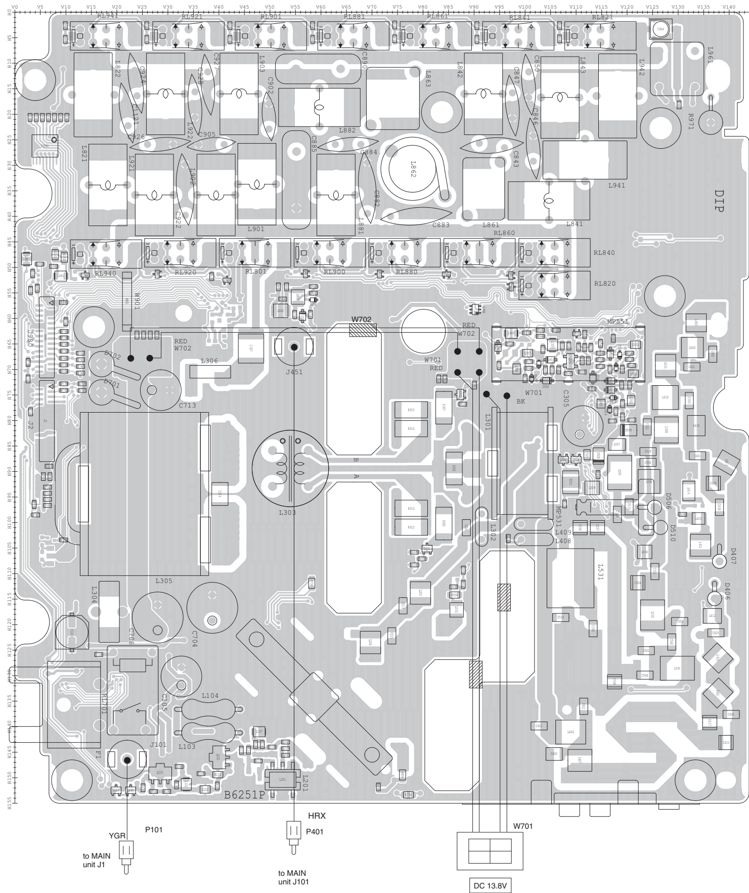
• PA UNIT (TOP VIEW)
